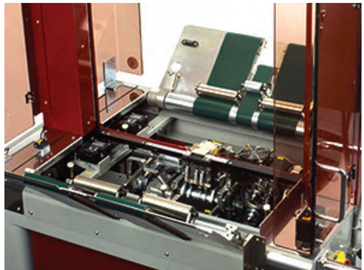
SIMPLIFIED STRAPPING HEAD WITH HINGED TOP PLATES
